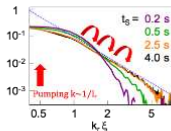
Fig.2 Cascade of turbulence for the momentum
