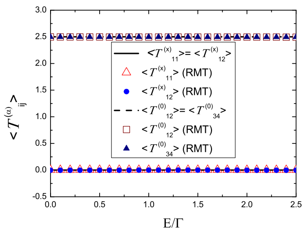
FIG. 2: (Color online) Generalized average transmission coefficient \langle \mathcal{T}_{ij}^{(\alpha)}(\epsilon, x=0) \rangle versus energy \epsilon = E/\Gamma for different spin and terminal indices. The analytical results (stub model) are represented by the solid and dotted lines, while the results of numerical simulations (RMT Hamiltonian model) are represented by the symbols. The figure inset describes the different \mathcal{T}_{ij}^{(\alpha)} .
