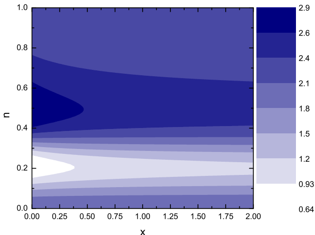
FIG. 4: [Color online] Contour plot of h_x(n, x) as a function of the magnetic field, represented by x , and the channel factor n . The color code is explained at the strip on the right panel.
