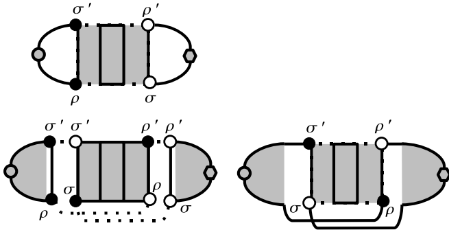
FIG. 1: Diagrams representing the leading contributions to the average transmission coefficient \langle \mathcal{T}_{ij}^{(\alpha)} \rangle of Eq. (7). Vertical lines represent contractions of the U matrix elements. The white and black dots stand for the channel indices of the matrix U and the Greek symbols represent the Pauli matrices indices \sigma_{\rho,\sigma} in the spin space. The first diagram (top) is known as diffuson and accounts for the semi-classical diffusive processes. The two others diagrams are known as cooperons and give the mean quantum correction, namely, the weak (anti)localization corrections.
