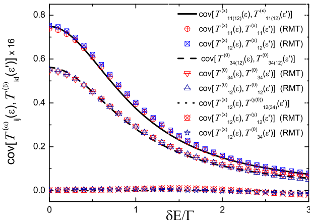
FIG. 3: (Color online) Transmission coefficient covariance \text{cov}[T_{ij}^{(\alpha)}(\epsilon, x=0)T_{kl}^{(\beta)}(\epsilon', x=0)] as a function of the energy difference \Delta\epsilon = (E - E')/\Gamma for different spin and terminal indices. The analytical results (stub model) are represented by the solid and dotted lines, while the results of numerical simulations (RMT Hamiltonian model) are represented by the symbols. The figure inset describes the different \text{cov}[T_{ij}^{(\alpha)}(\epsilon)T_{kl}^{(\beta)}(\epsilon')] considered.
