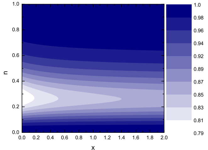
FIG. 5: [Color online] Contour plot of h_\epsilon(n, x) as a function of the magnetic field, represented by x , and the channel factor n . The color code is explained at the strip on the right panel.
