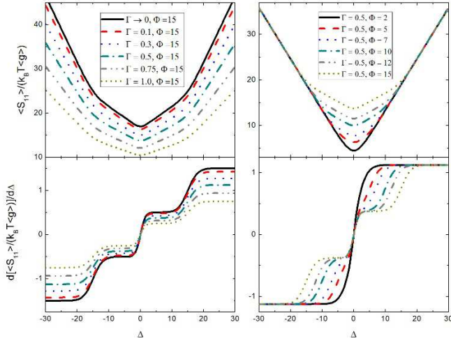
FIG. 2: We depict the behavior of the noise and its first derivative in the regime of spin accumulation as a function of tunneling rate \Gamma in a quantum dot with non-ideal symmetrical contacts. For \Delta > \Phi , We observe that the noise suffers abrupt changes, enhanced by the finite tunneling rates.
