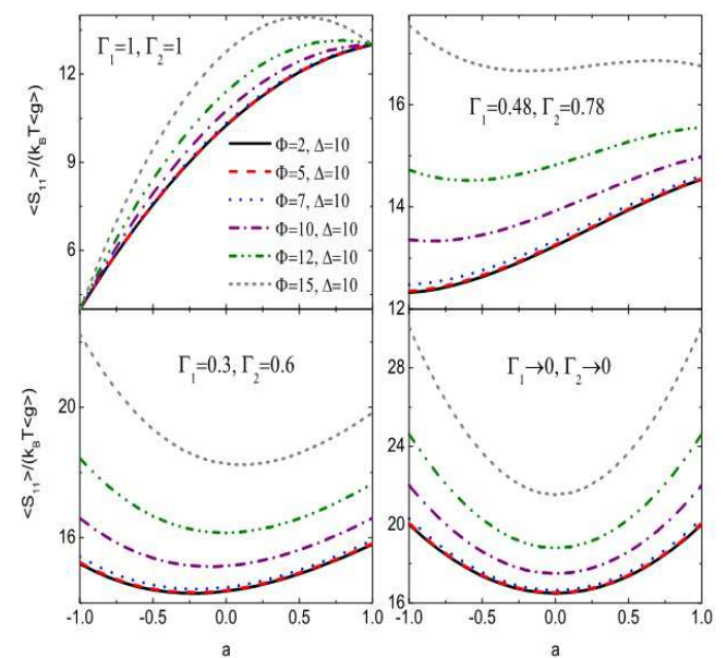
FIG. 3: We depict the behavior of the noise in the regime of spin accumulation as a function of the tunneling rate \Gamma in a QD with non-ideal contacts, through the parameter a = (G_1 - G_2) / G_T . Note that for ideal contacts, \Gamma_1 = \Gamma_2 = 1 , the noise is highly asymmetrical with respect to this parameter. In the other curves we vary the values of \Gamma_1 and \Gamma_2 till we reach the opaque limit, \Gamma_{1,2} \rightarrow 0 . In this case the noise becomes symmetrical with respect to a .
