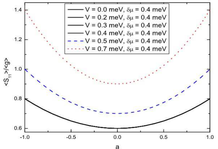
FIG. 5: We show the behavior of the shot noise in the case of spin accumulation as a function of a = (G_1 - G_2)/G_T , in a QD with non-ideal contacts, equation (13). For any value such that \delta\mu \geq eV , the result will always be the same for the shot noise which is a direct consequence of the spin accumulation in the reservoirs.
