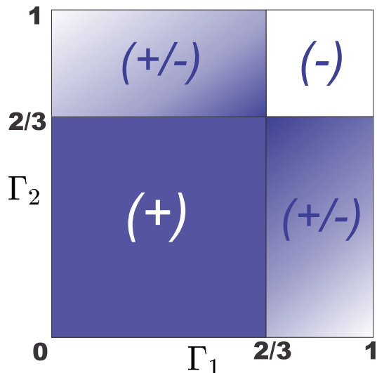
FIG. 4: In this figure we show the concavity and the sign of the noise power for all values of the tunneling rate and of the asymmetry parameter.
