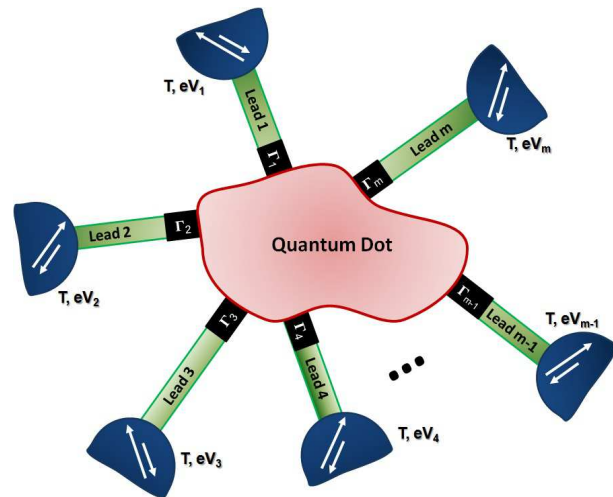
FIG. 1: A schematic picture showing a quantum dots coupled to polarizable reservoirs via several leads with open channels in the presence of temperature and voltage.
